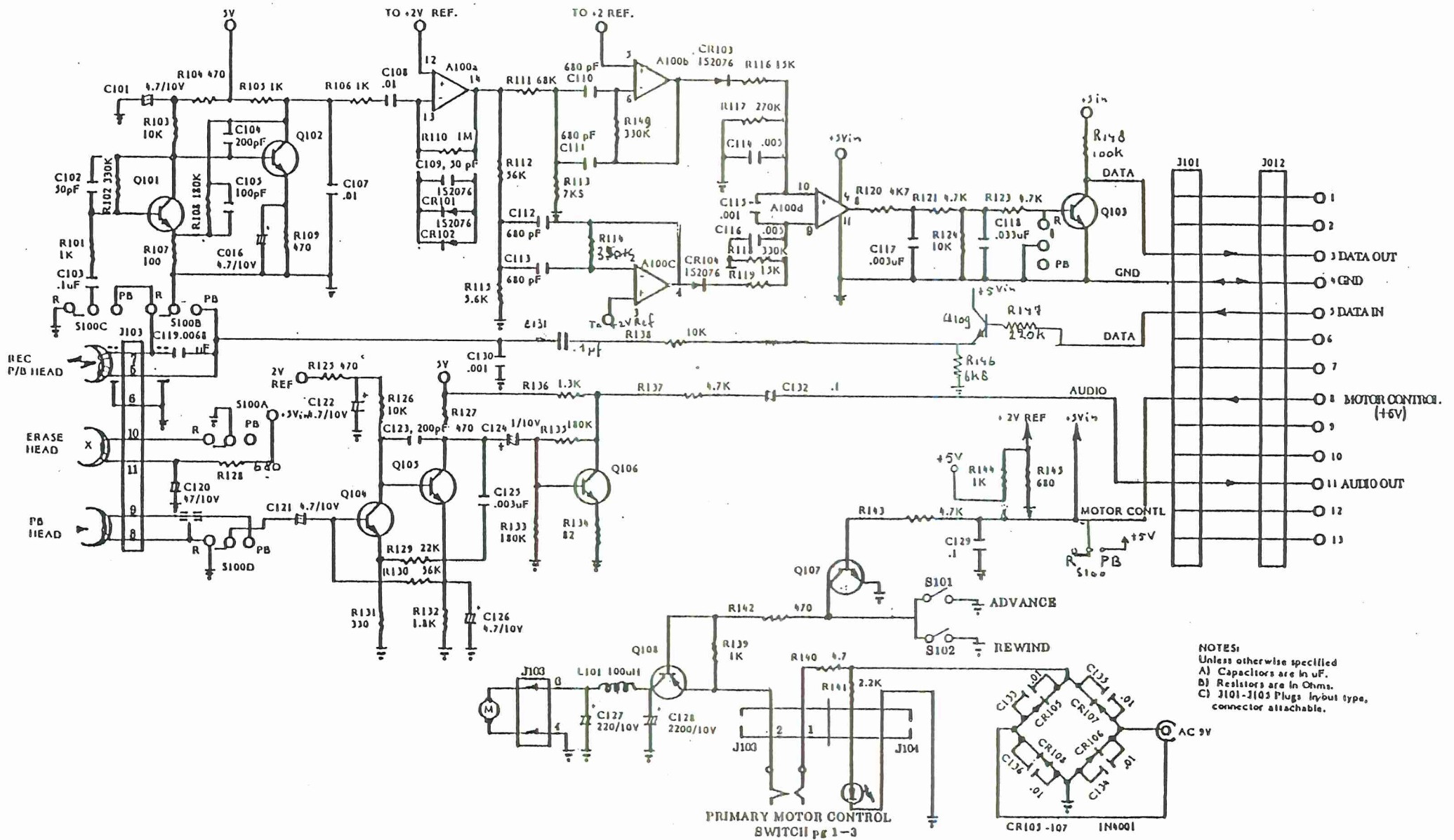
1010C Schematic
