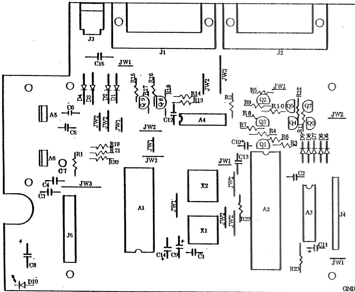
Figure 2-1. 1020 Color Printer Silkscreen.
