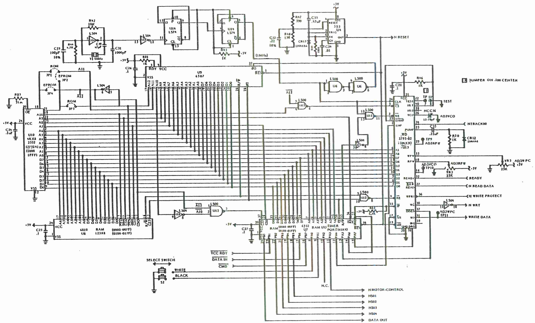
1050 Schematic (Tandon) 2 of 4
